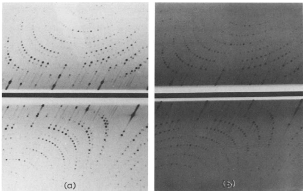
Fig. 1. Weissenberg photographs, showing the effect of anomalous scattering. (-)_589\text{-}\Delta\text{-[Co-(S,S-chxn)}_3\text{]Cl}_3 \cdot 5\text{H}_2\text{O} . a -axis rotation, O-th layer. (a) Taken with Fe K\alpha radiation ( \lambda = 1.937 \text{ \AA} ) (b) Taken with Cu K\alpha radiation ( \lambda = 1.542 \text{ \AA} ).
