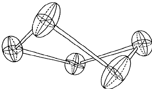
Fig. 4. View of thermal motion ellipsoids of a Co-en ring.
